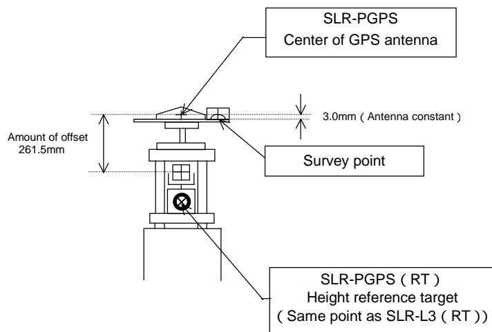
Figure 7. GPS antenna for SLR geodetic survey (1998 Tateyama)
