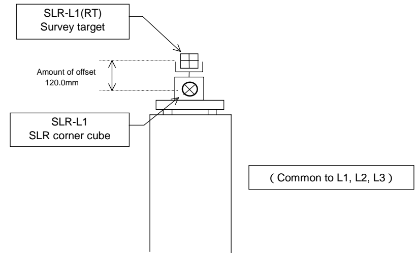
Figure 2. SLR external geodetic survey reference point (long pillar)
