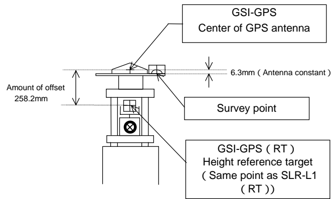
Figure 13. GSI-GPS electronic reference point (1999 Koganei)
