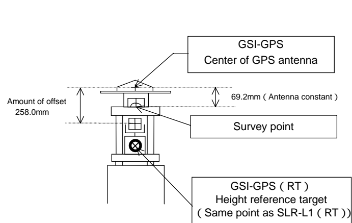
Figure 9. Ground reference point for satellite geodetic survey No.4 (Koganei station)
