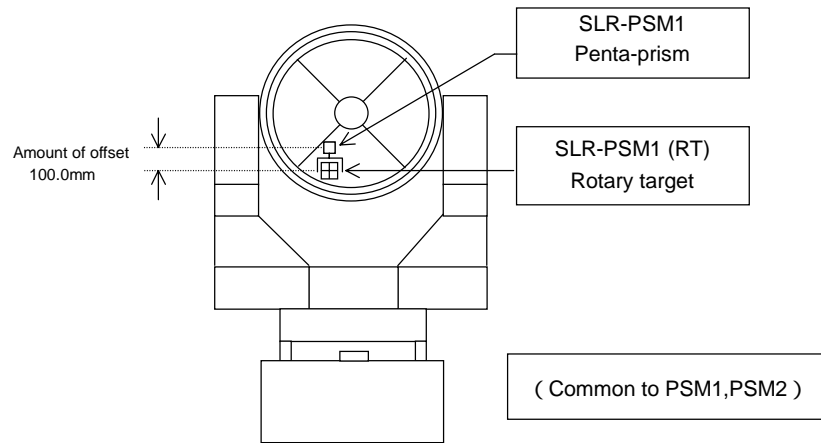
Figure 5. SLR prism
