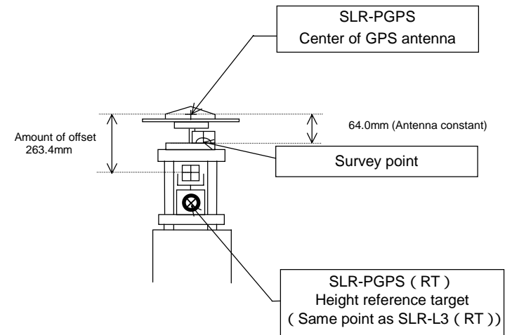
Figure 8. GPS antenna for SLR geodetic survey (1999 Tateyama)
