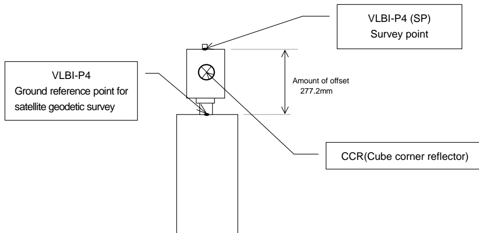
Figure 9. Ground reference point for satellite geodetic survey No.4 (Koganei station)
