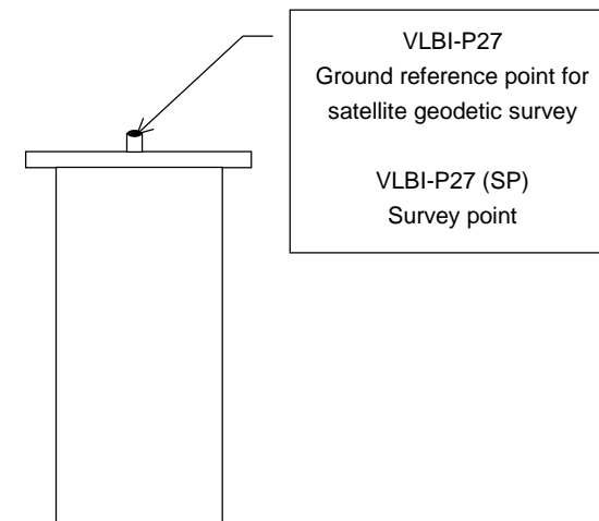
Figure 10. Ground reference point for satellite geodetic survey No.27 (Koganei station)
