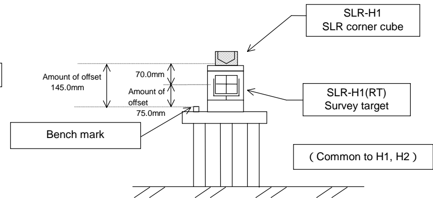
Figure 4. SLR leveling reference point
