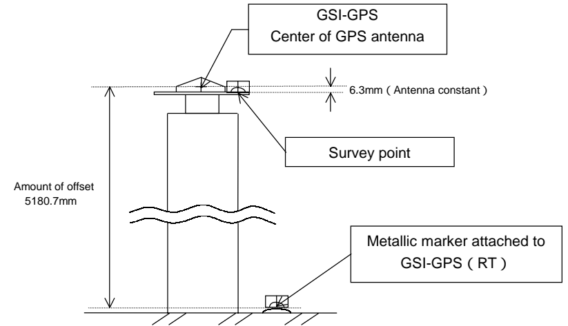
Figure 14. GSI-GPS electronic reference point (1999 Kashima)
