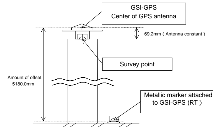
Figure 10. Ground reference point for satellite geodetic survey No.27 (Koganei station)
