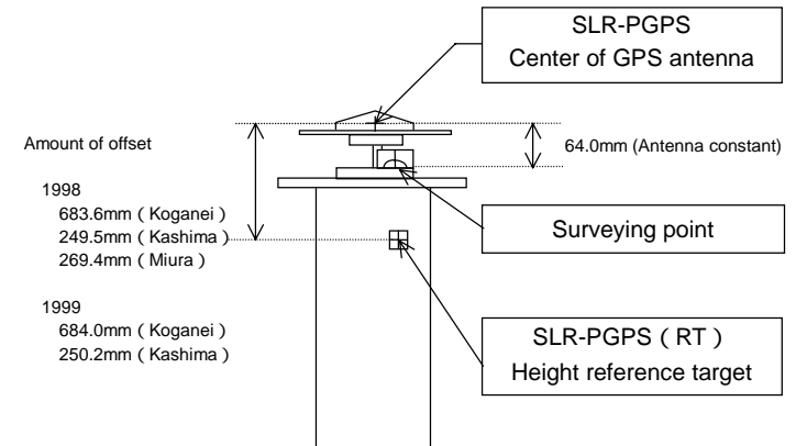
Figure 6. GPS antenna for SLR geodetic survey (Koganei, Kashima, Miura)
