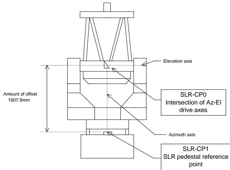
Figure 1. SLR telescope reference point
